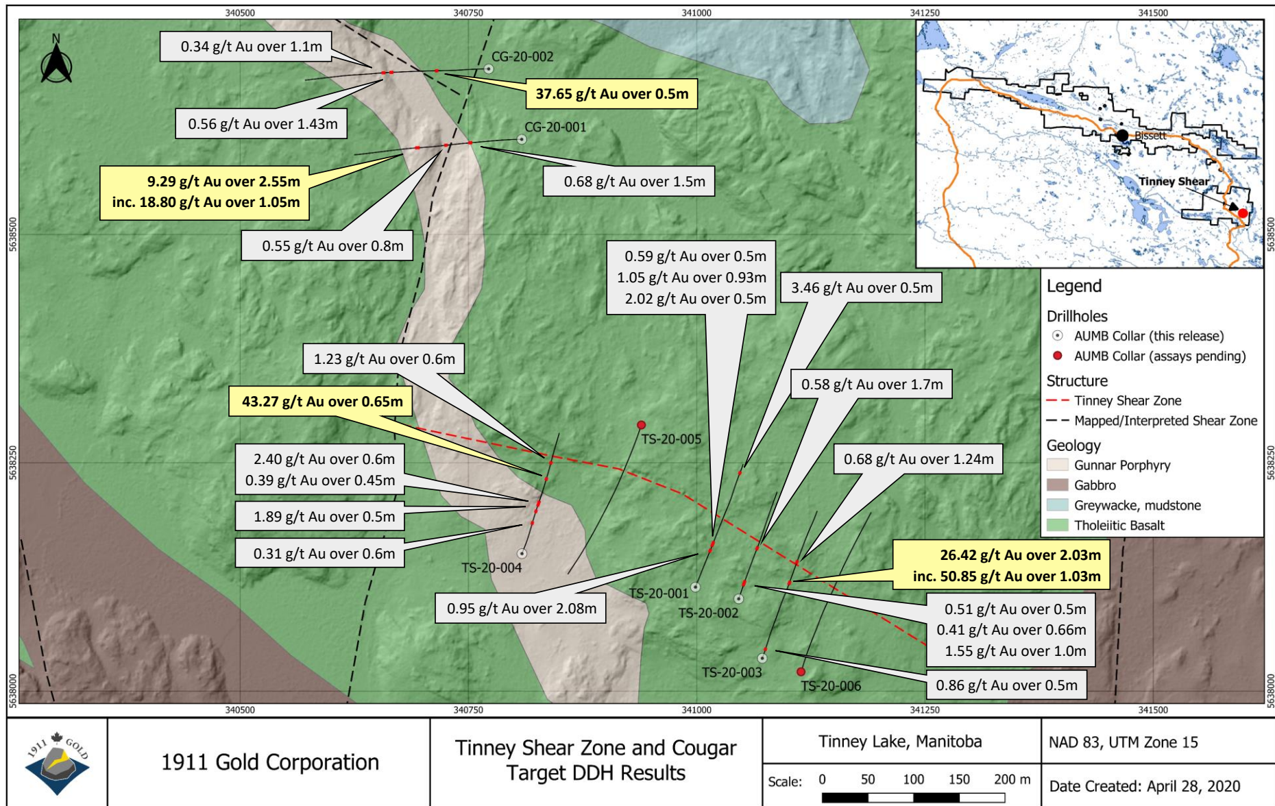
Figure 2: Plan map of the Tinney Shear (TS) and Cougar (CG) targets, showing drillhole locations and major shear zones. Map base is a shaded-relief LiDAR DEM with bedrock geology drape.
