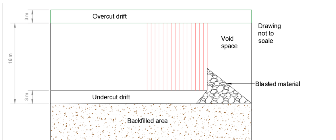
Figure 16.13 Longhole open stope blasting
