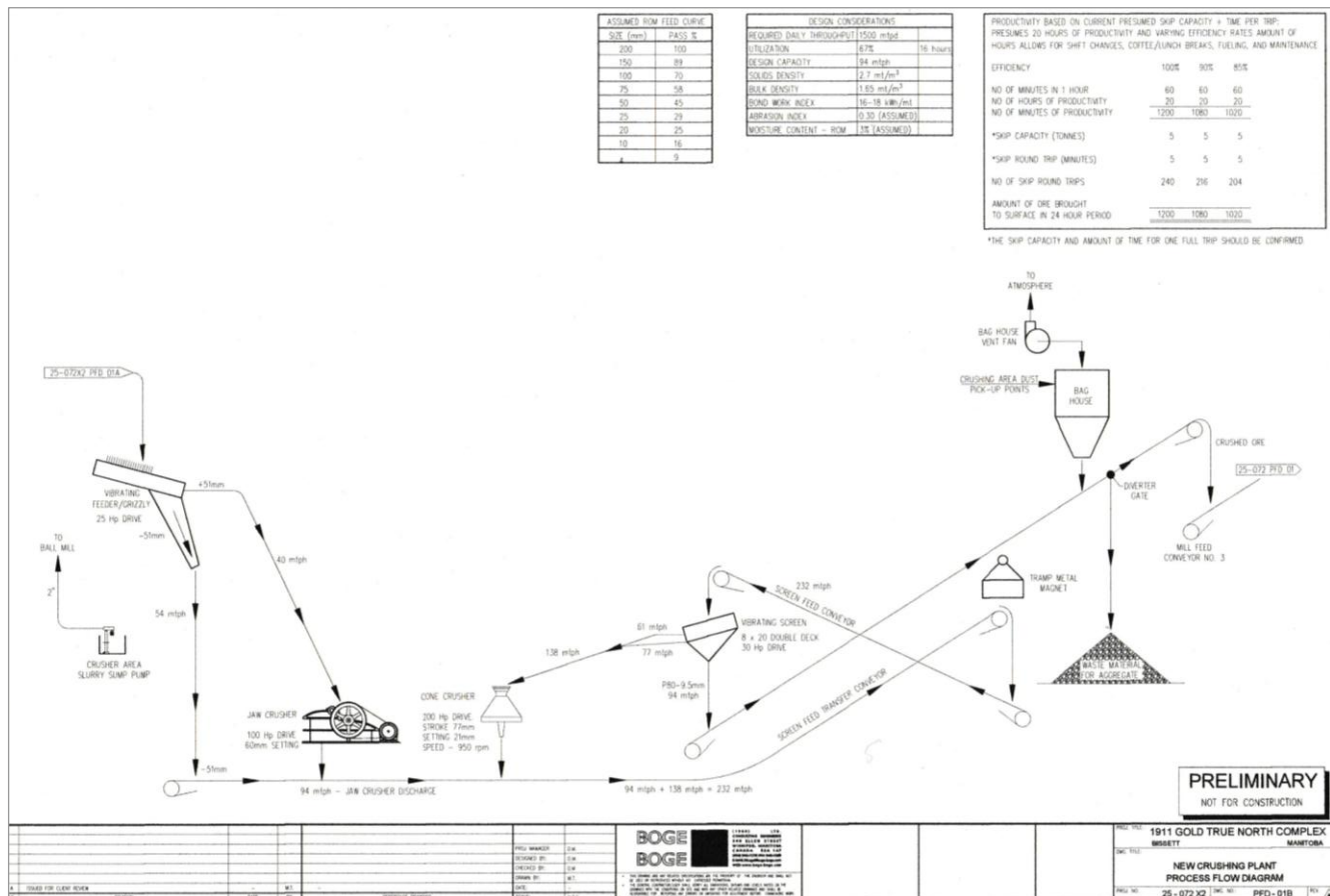
Figure 17.1 1911 Gold processing plant – crushing circuit
