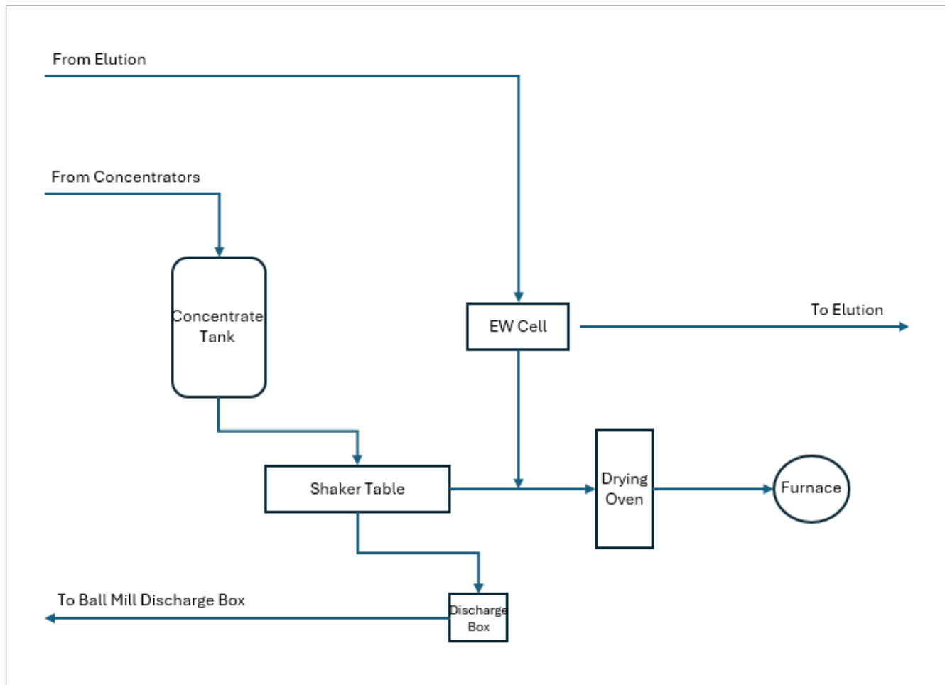
Figure 17.7 1911 Gold processing plant – refinery circuit
