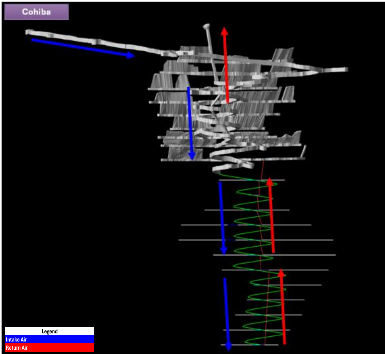
Figure 16.7 Conceptual ventilation flow – Cohiba (looking north)
