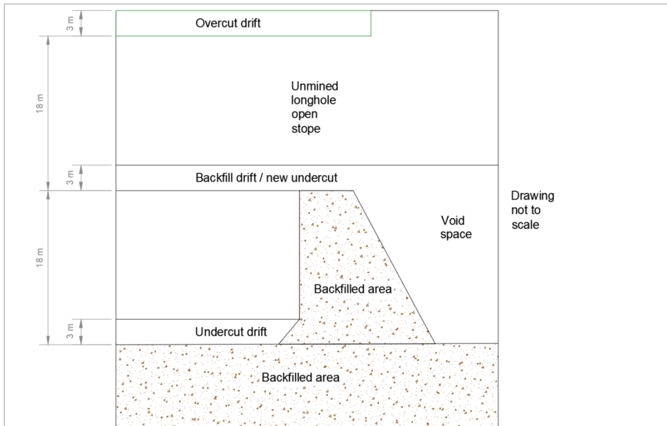
Figure 16.14 Longhole open stope backfilling
