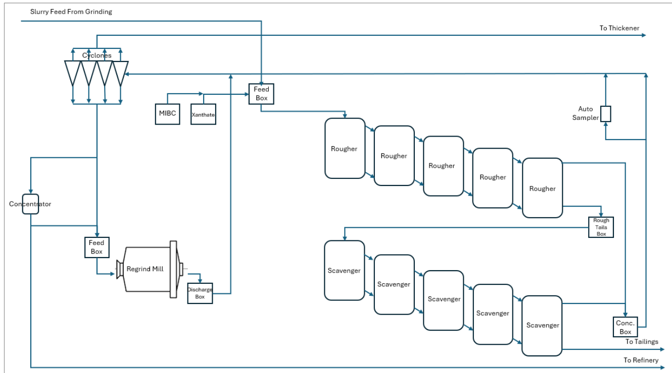
Figure 17.3 1911 Gold processing plant – flotation circuit
