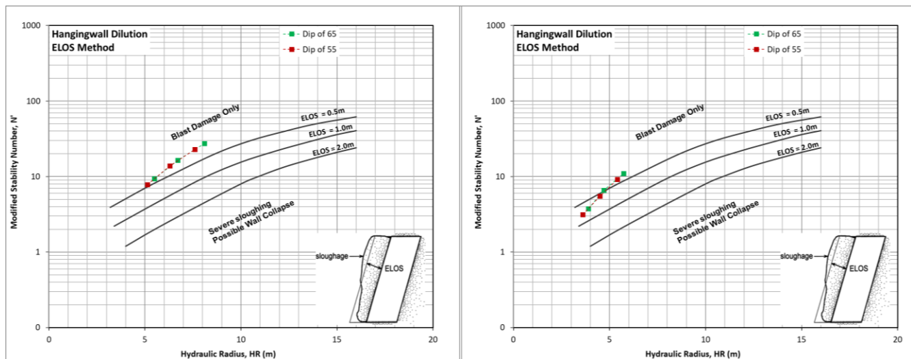
Figure 16.3 Estimated ELOS for currently anticipated rock mass conditions (left: average structure conditions; right: adverse structure conditions)
