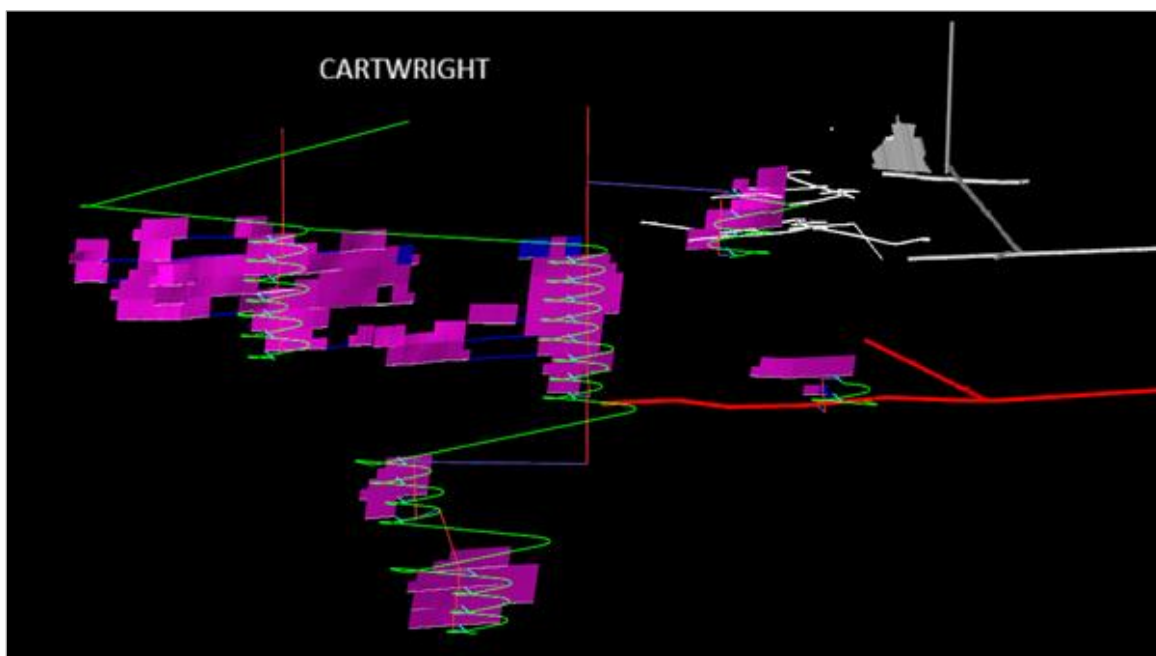
Figure 16.16 Cartwright underground mine design (looking north)
