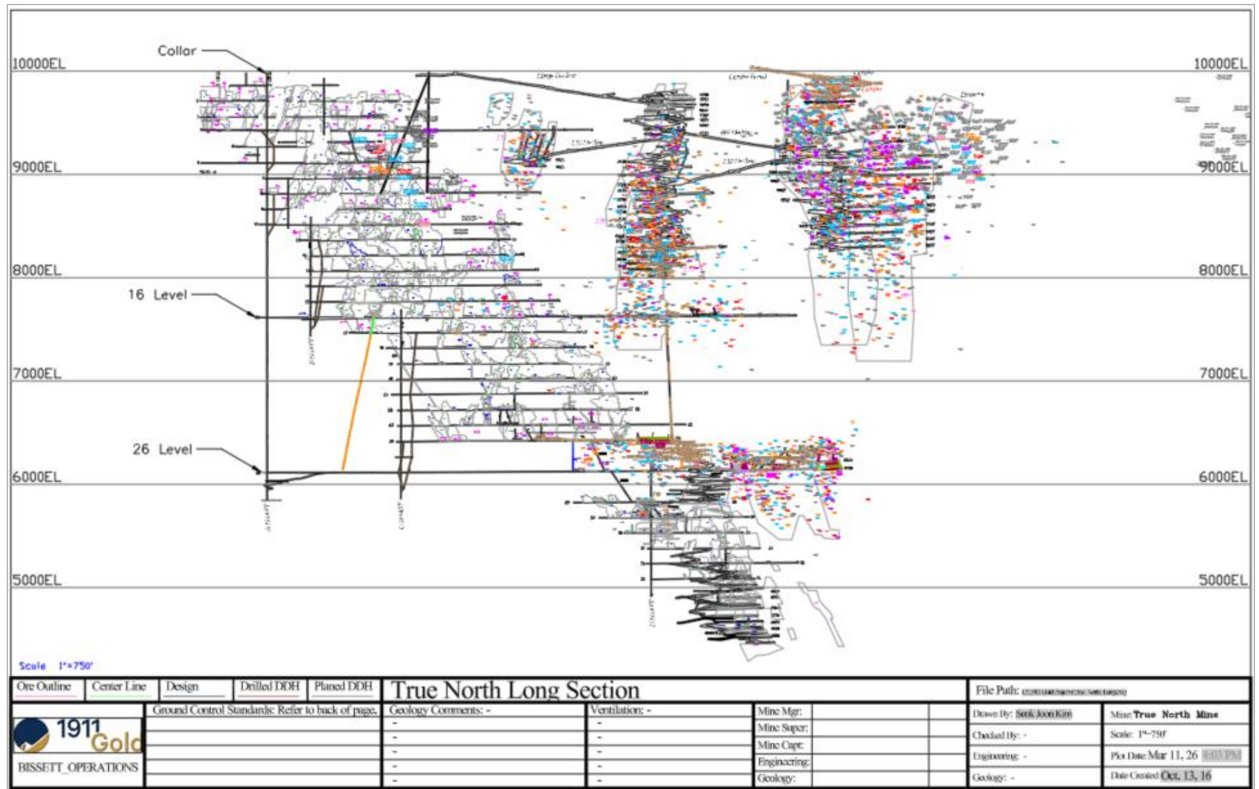
Figure 16.4 Longitudinal section (looking north)
