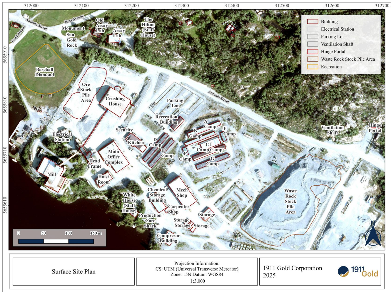
Figure 5.4 Plan view of mine surface infrastructures
