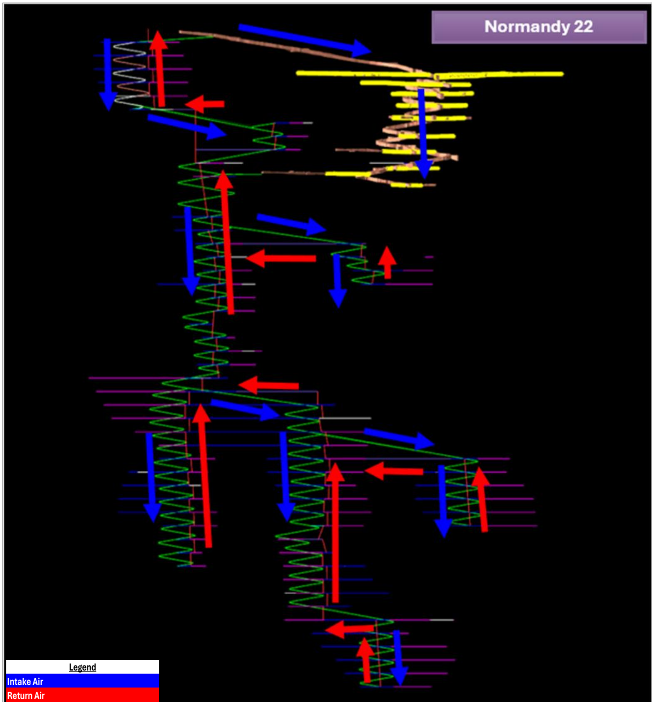
Figure 16.8 Conceptual ventilation flow – Normandy 22 (SG-1) (looking north)
