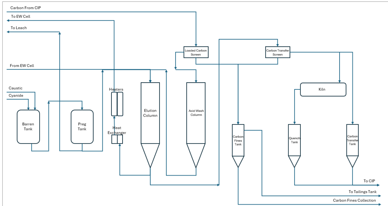
Figure 17.6 1911 Gold processing plant – elution circuit
