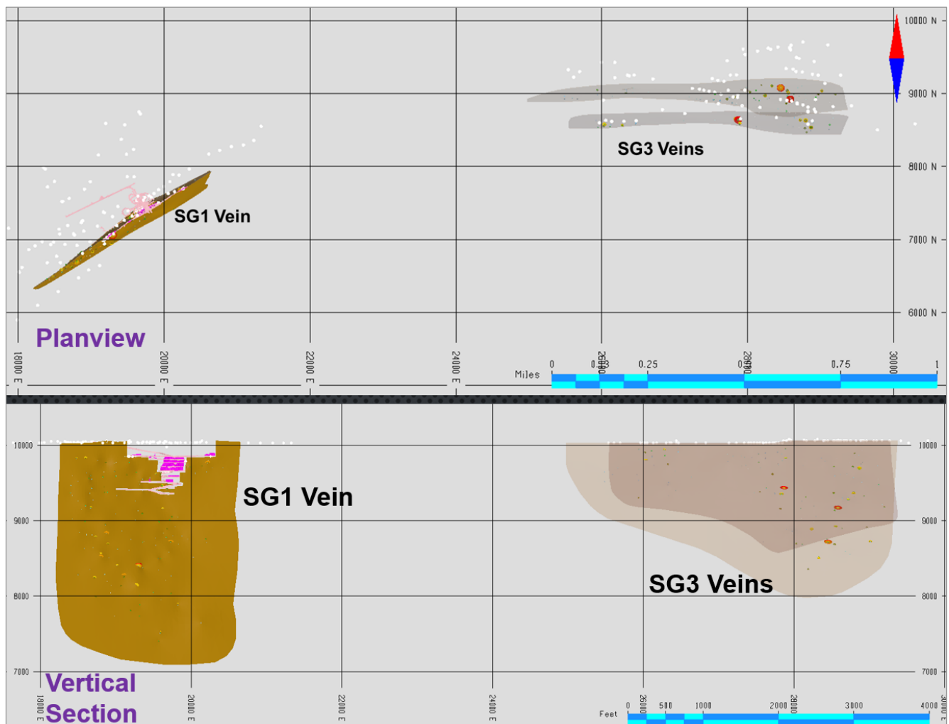
Figure 14.11 Planview and vertical east-west section (looking North) of the Normandy Zone vein domains
