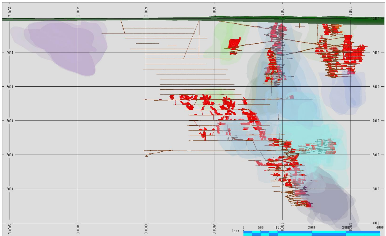
Figure 14.4 Longitudinal section (looking north) with historical mined stopes, drift, and shaft locations in the areas of MRE
