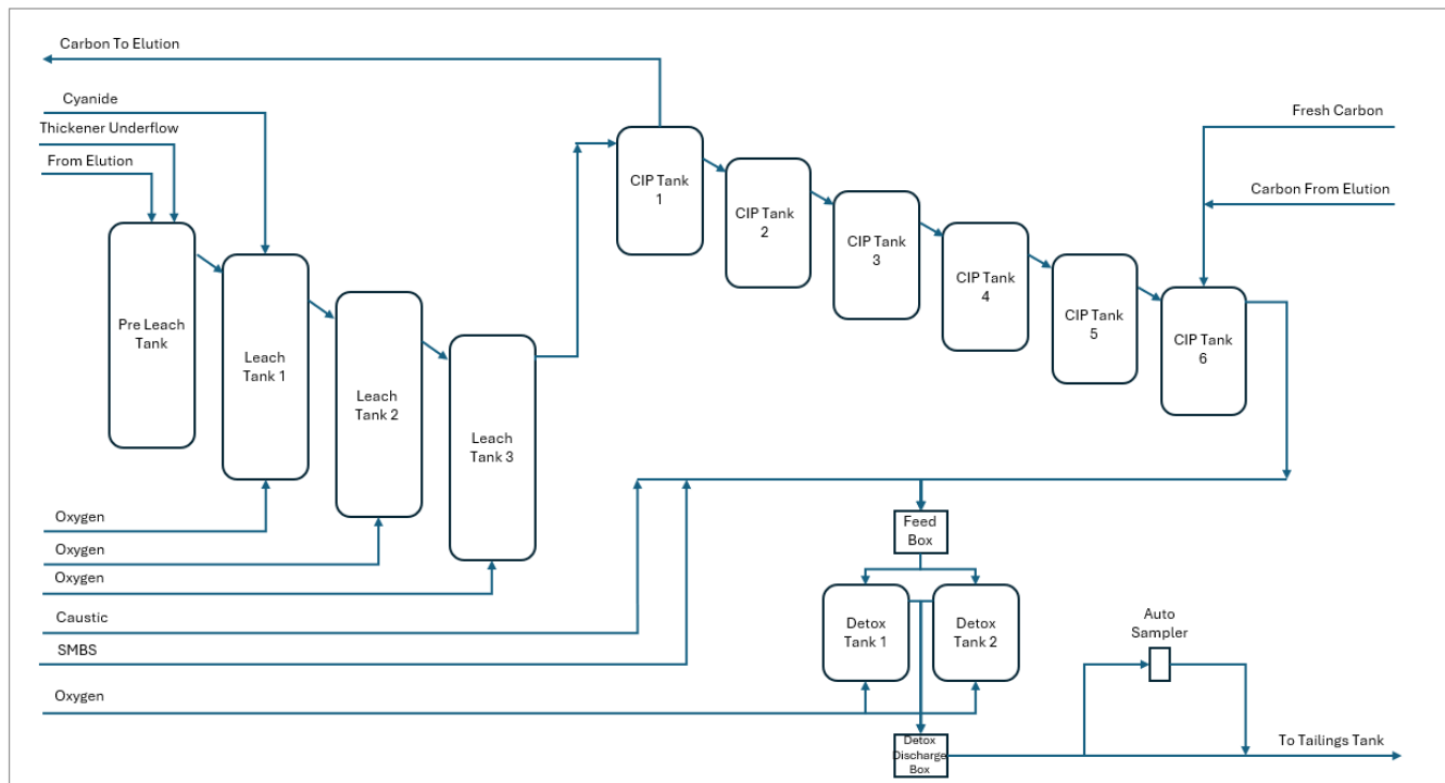
Figure 17.5 1911 Gold processing plant – cyanide leaching circuit
