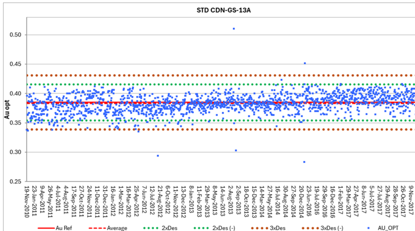
Figure 11.1 Gold CRM CDN-GS-13A
