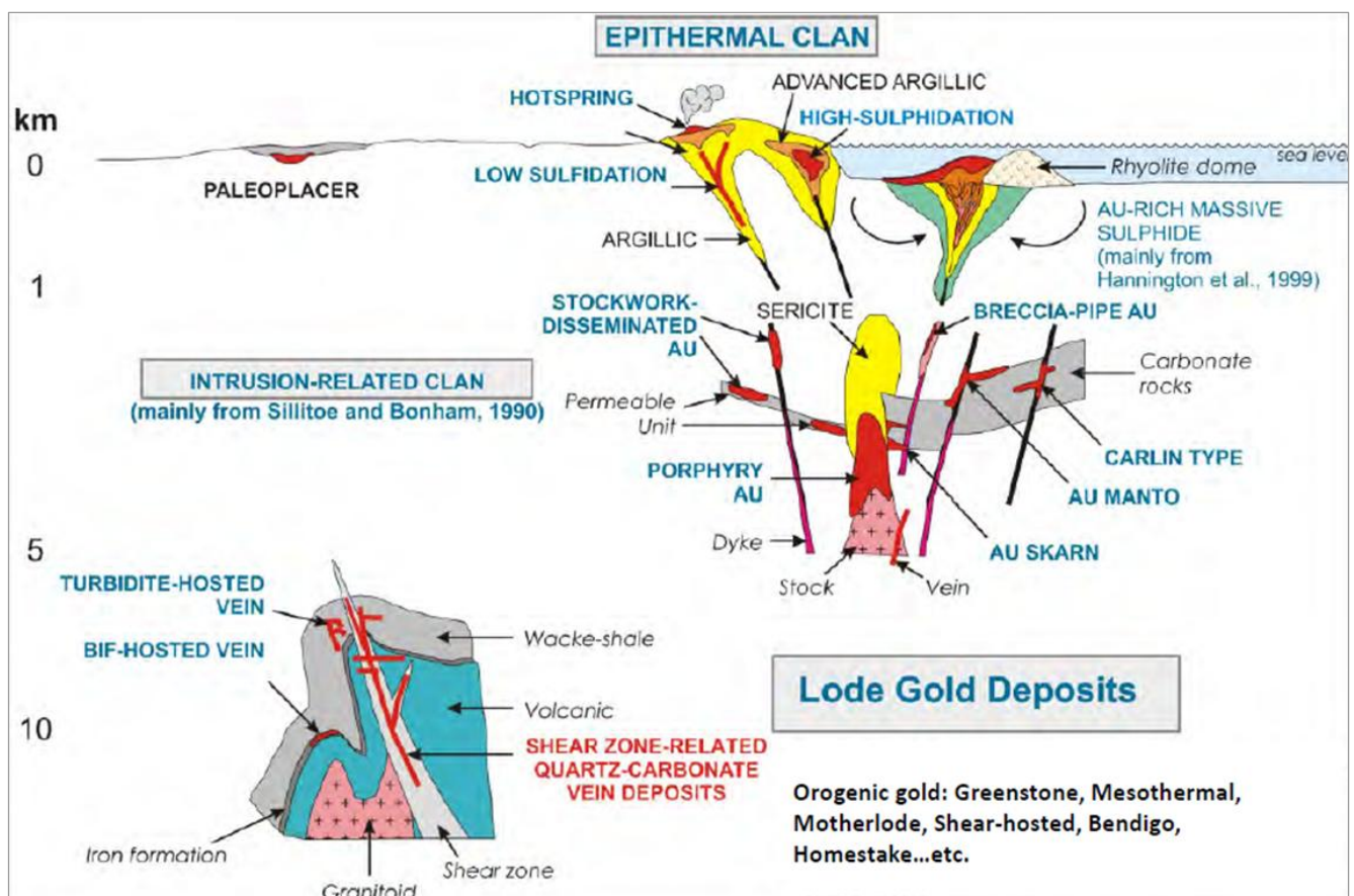
Figure 8.1 Schematic cross-section representation of the geometry and structural setting of shear zone hosted gold-bearing quartz vein networks in greenstone belt terrains like True North Gold deposits
