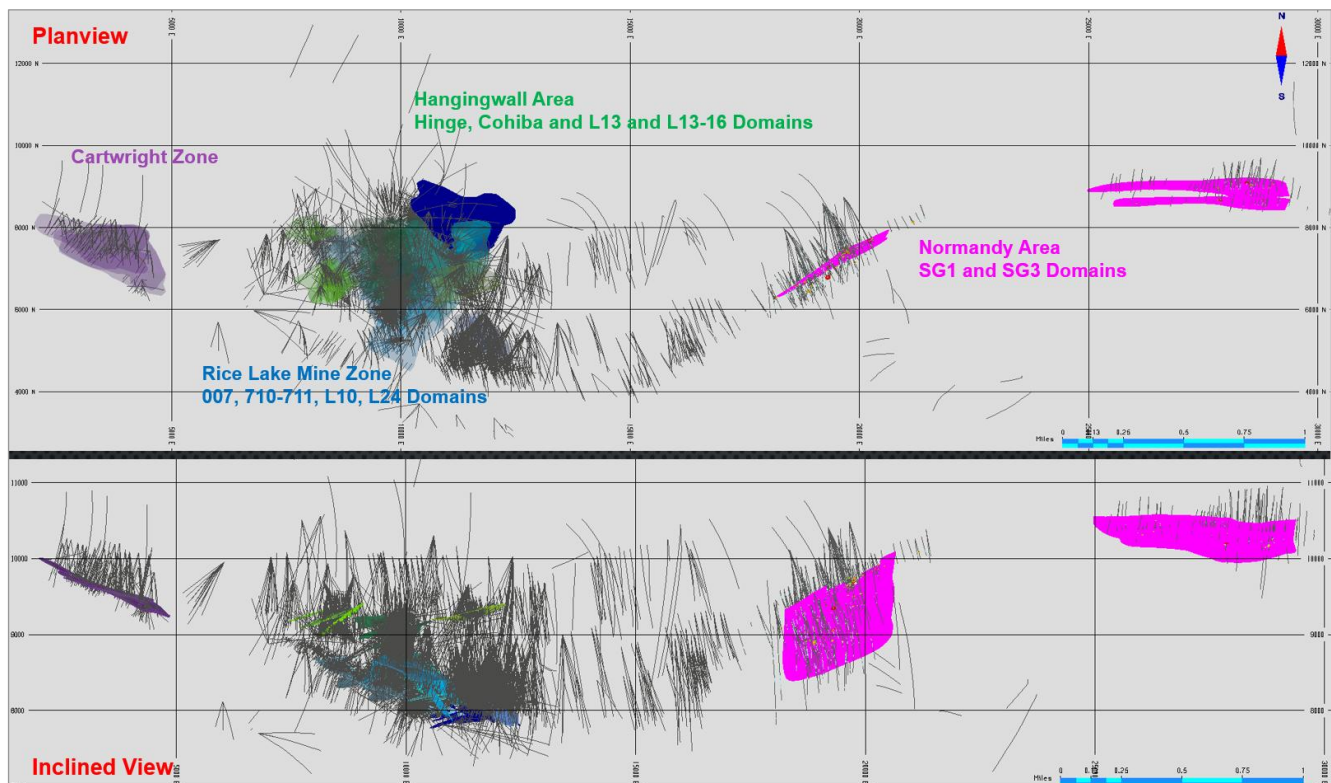
Figure 14.1 Plan view and inclined view of all drillholes in the True North Gold Deposit database
