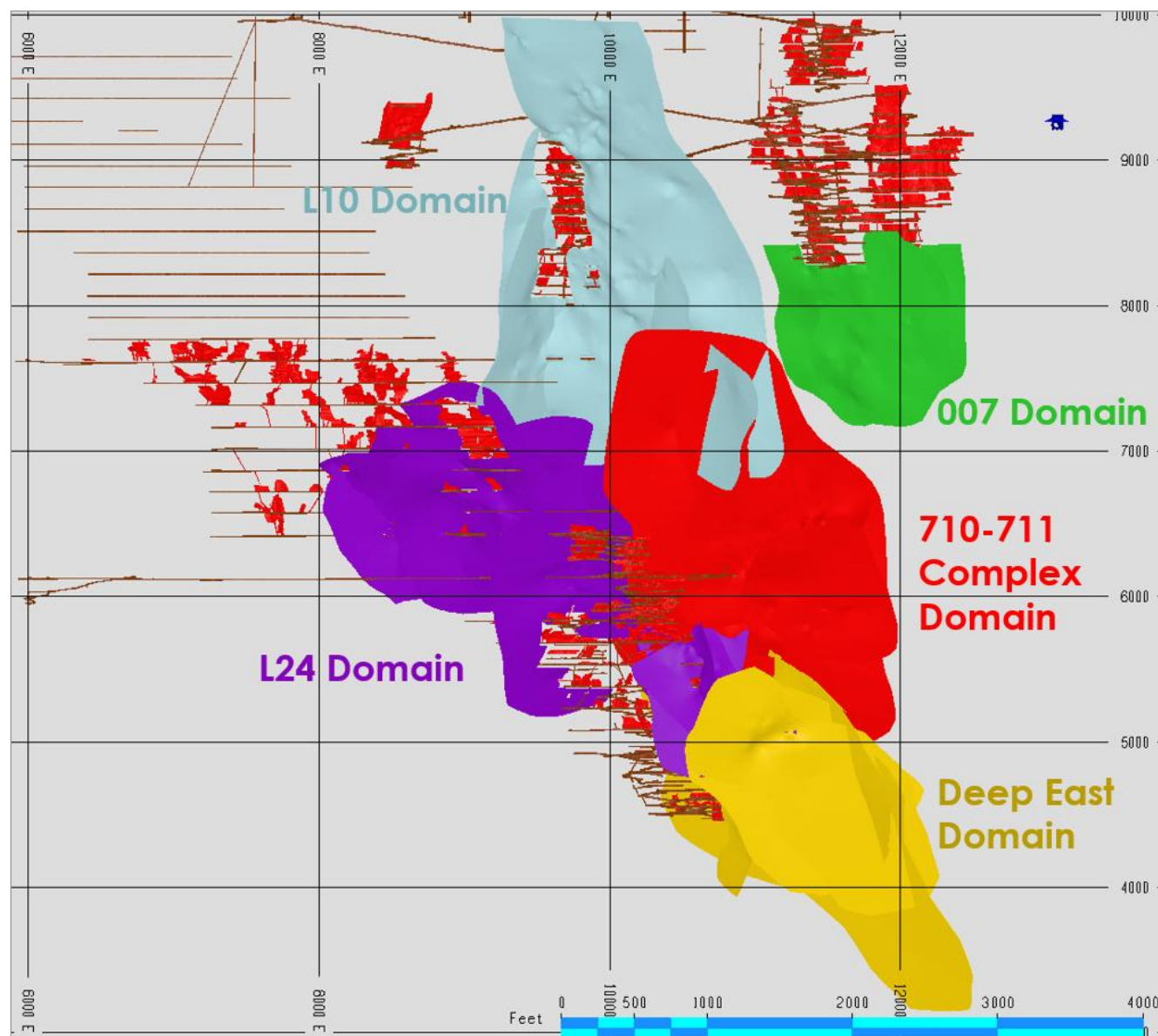
Figure 14.10 EW vertical section (looking north), Rice Lake Mine Zone vein domains with vein solids and underground infrastructure
