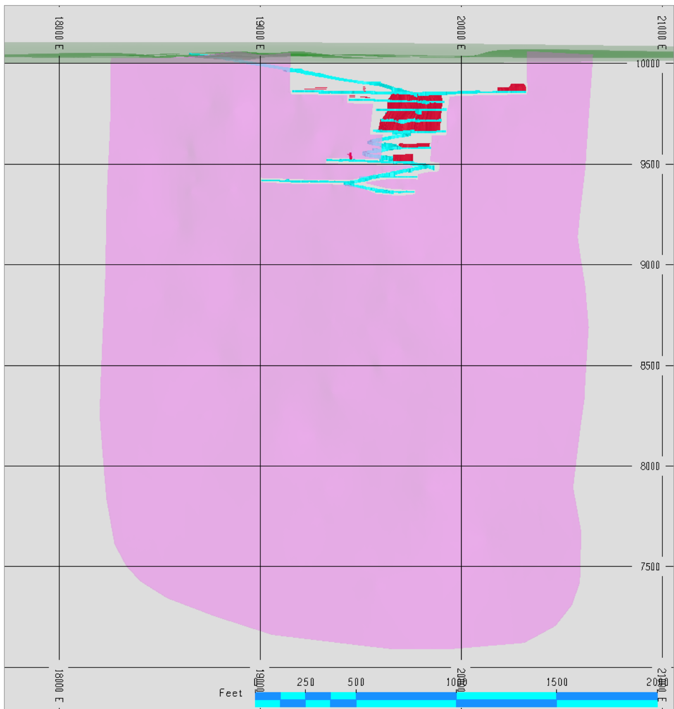
Figure 14.5 Longitudinal section (looking north) with historical mined stopes, drift, and shaft locations at Normandy Zone, SG1 vein domain in the areas of the MRE
