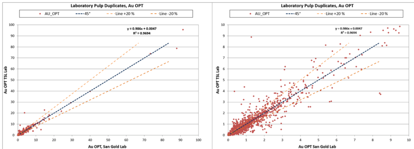
Figure 11.3 Laboratory pulp duplicates, scatter plot, Au OPT
