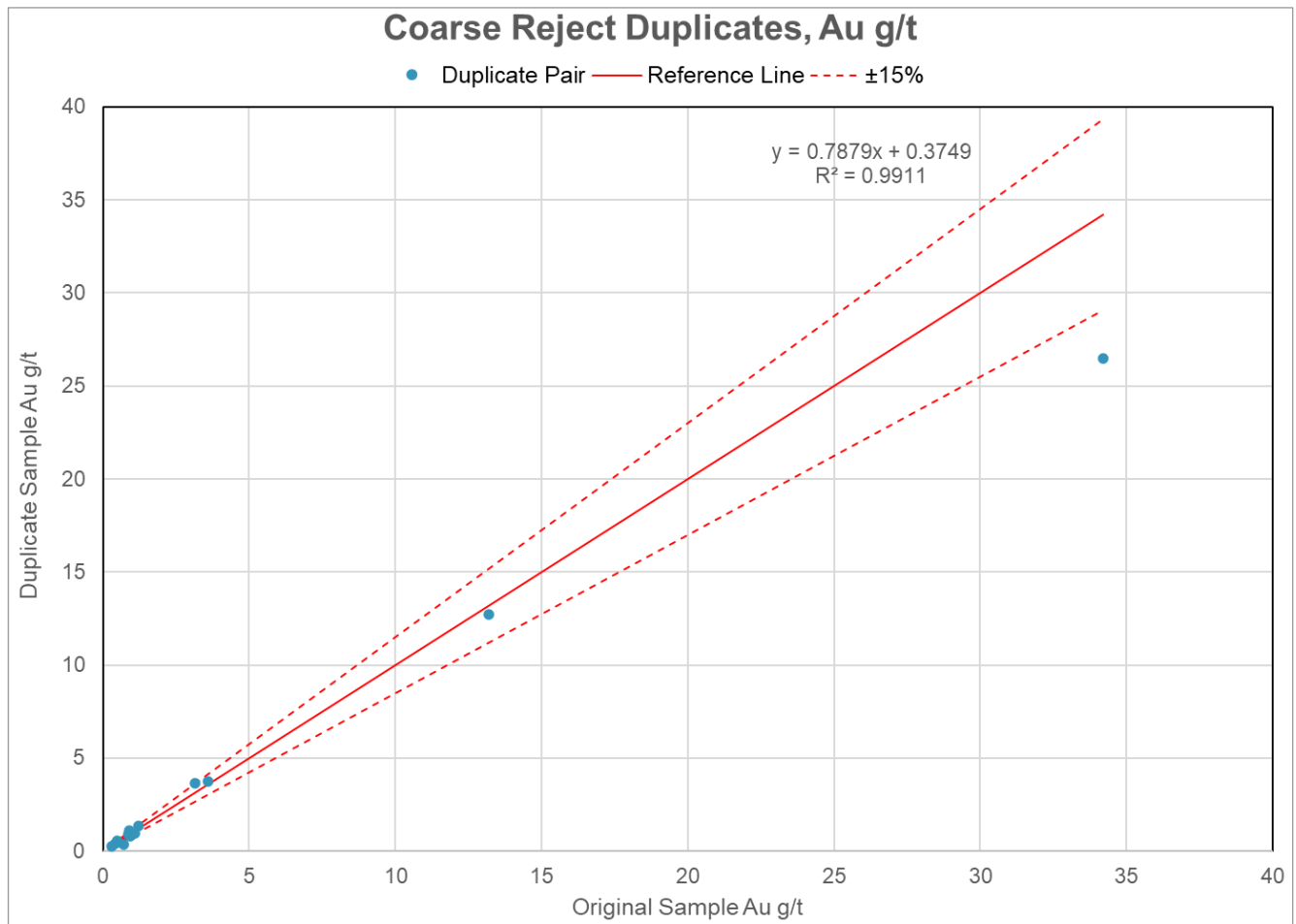
Figure 11.5 Coarse reject duplicates, scatter plot, Au g/t
