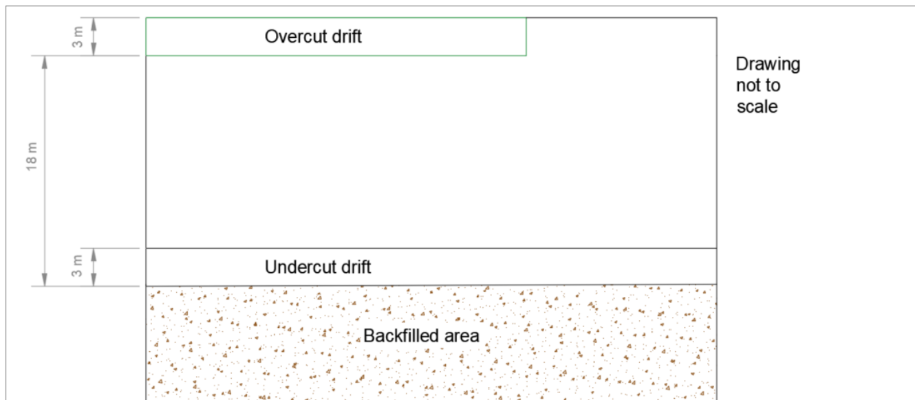
Figure 16.11 Longhole open stope sill development
