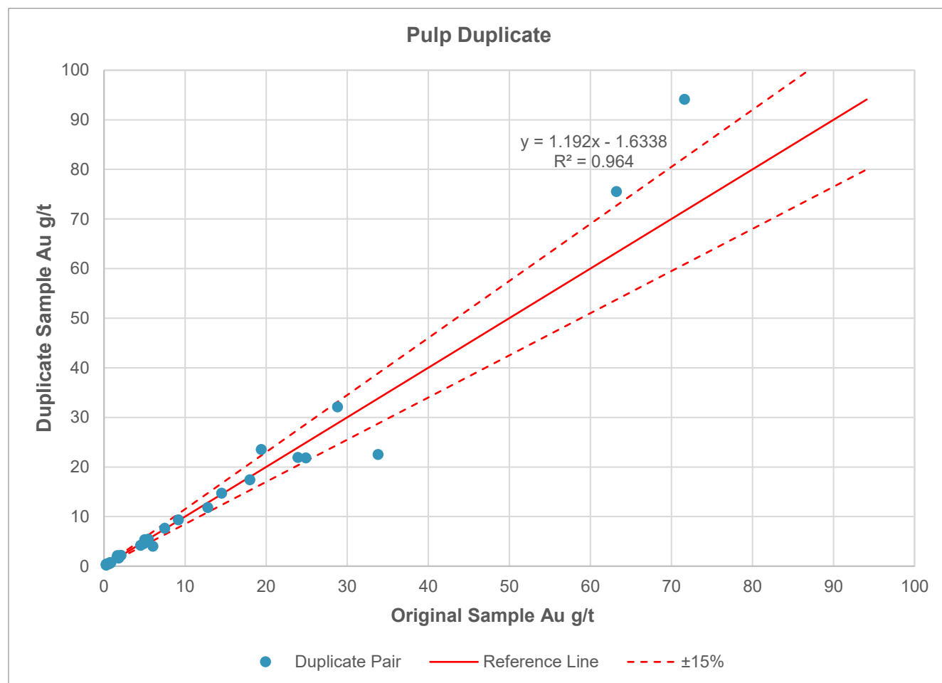
Figure 11.6 Pulp duplicates, scatter plot, Au g/t
