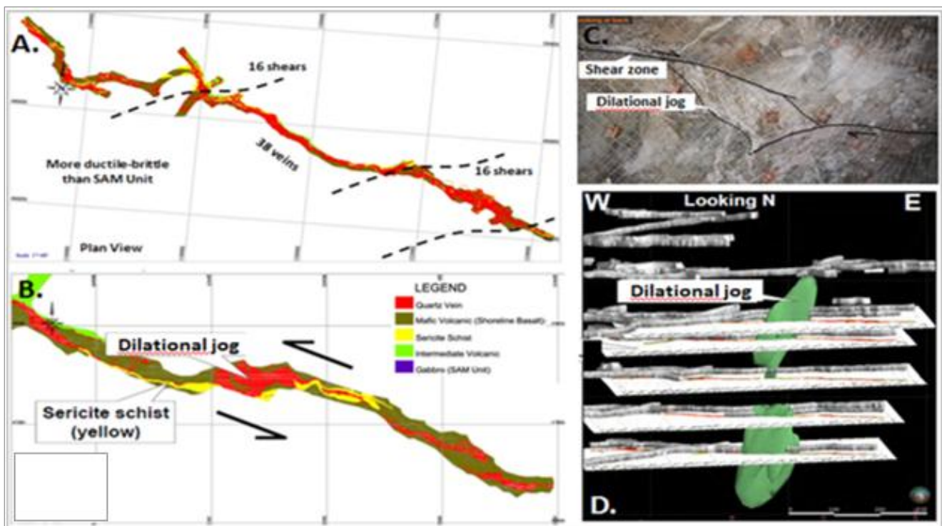
Figure 7.11 Controls on gold mineralization in the 007 Zone
