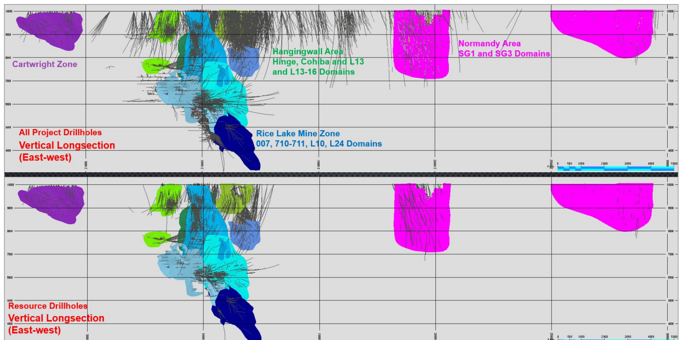
Figure 14.3 Vertical east-west sections (looking north) showing all drillholes in the project database (top) and drillholes used for the MRE (bottom)
