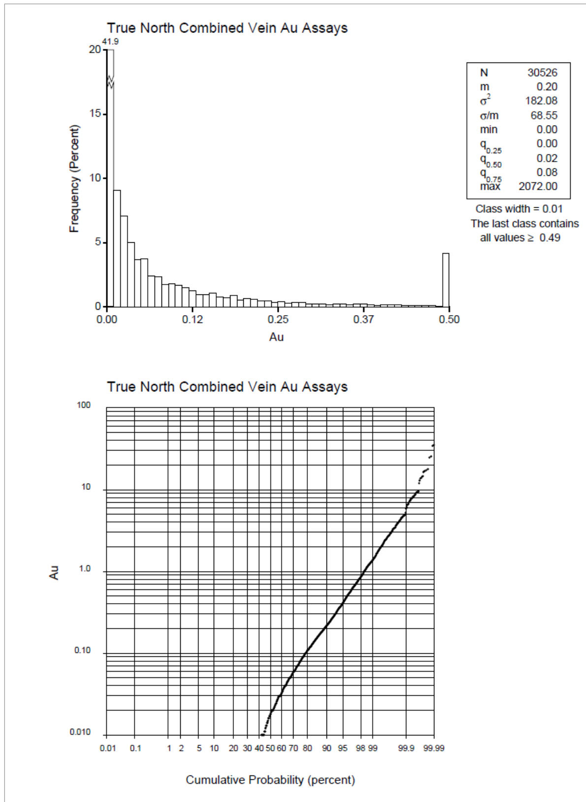
Figure 14.6 Histogram / probability plot of all assay data within vein solids, Au oz/st
