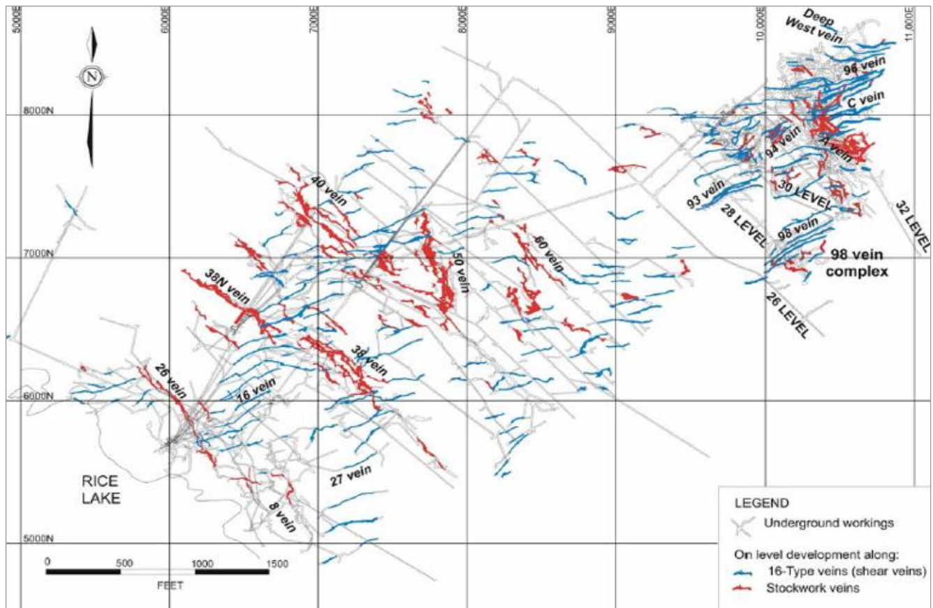
Figure 7.8 Distribution of 16-type (shear) veins and 38-type (stockwork veins) on composite plan of mine working in the True North Mine
