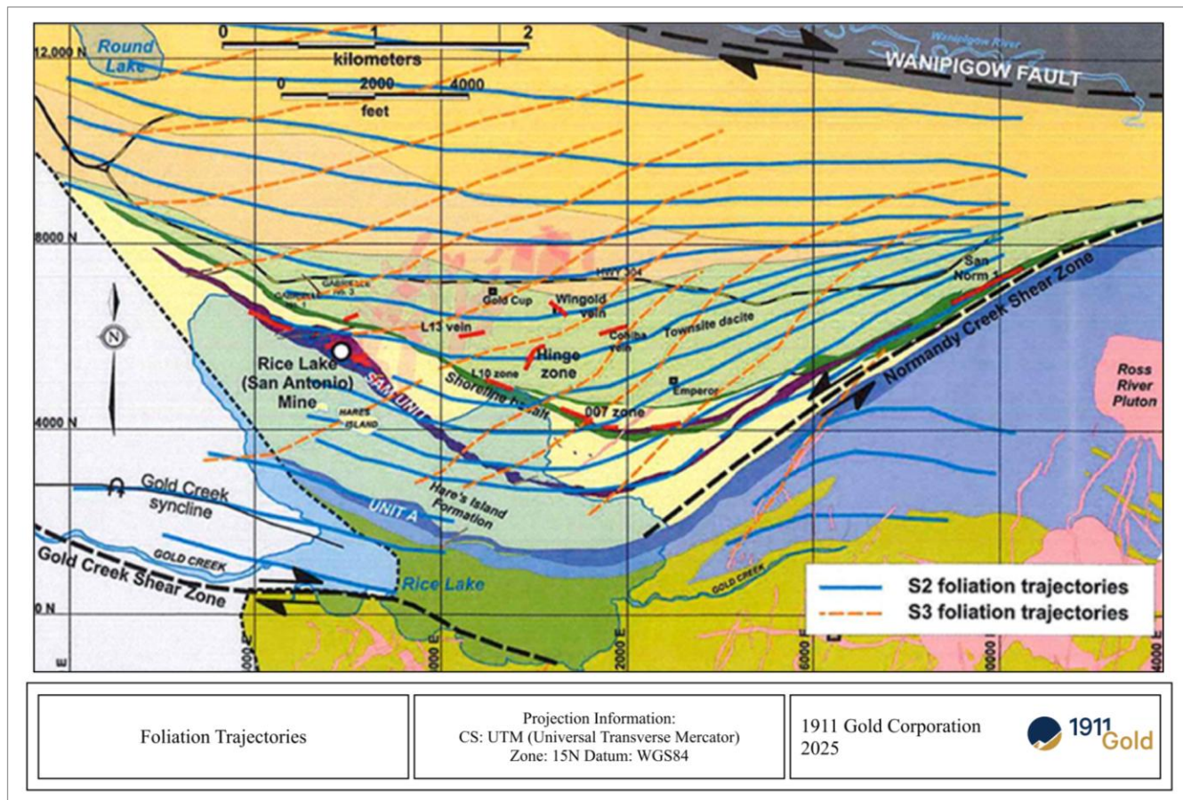
Figure 7.5 The structural geological setting S2 and S3 foliation trends
