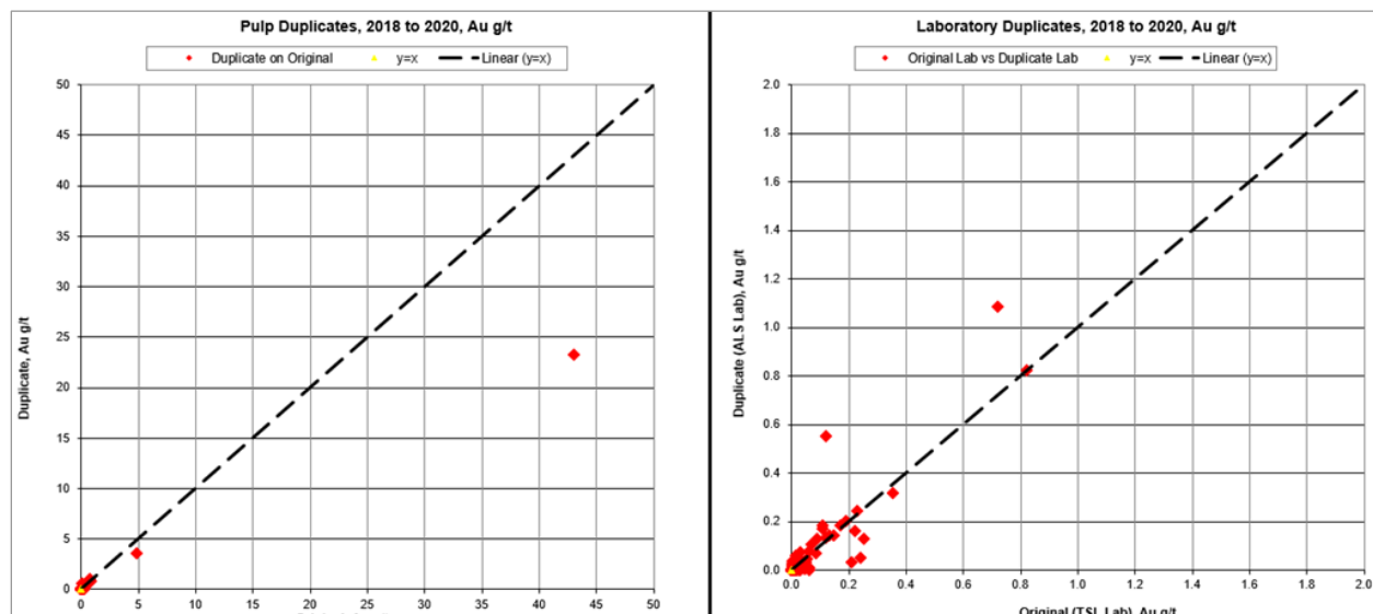
Figure 11.4 Laboratory pulp duplicates for 2018 to 2020, Au g/t
