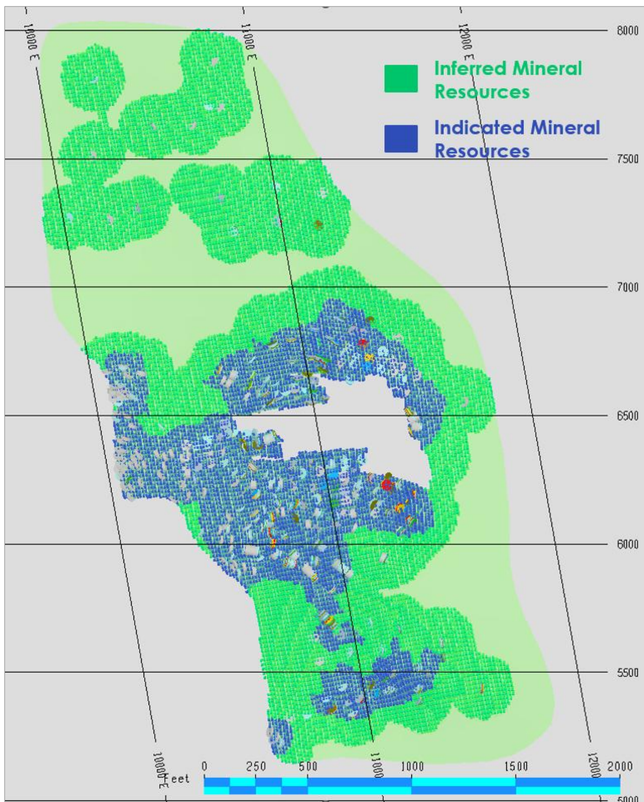
Figure 14.16 Vertical section (looking north), classification of 710-711 Complex Zone, 710 Vein
