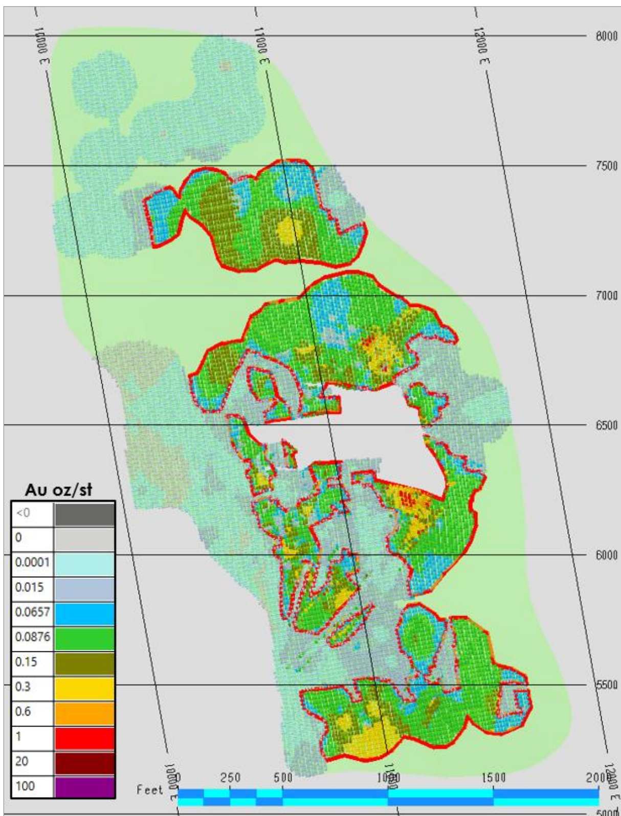
Figure 14.17 Vertical section (looking north), 710-711 Complex Zone, 710 Vein, 0.0657 oz/st Au (2.25 g/t Au) Mineral Resource constraining envelopes (red outline)
