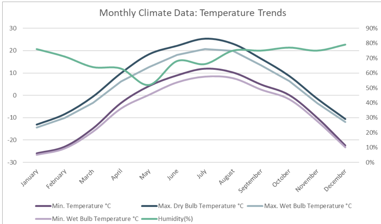
Figure 16.5 Monthly surface climate conditions
