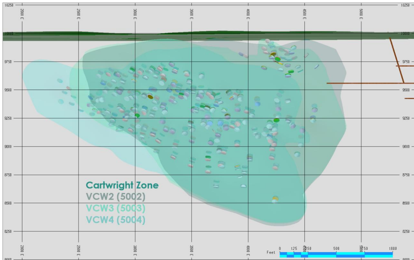
Figure 14.7 Vertical section (looking north), Cartwright Zone showing location of veins, infrastructure, topography, and drillhole composites
