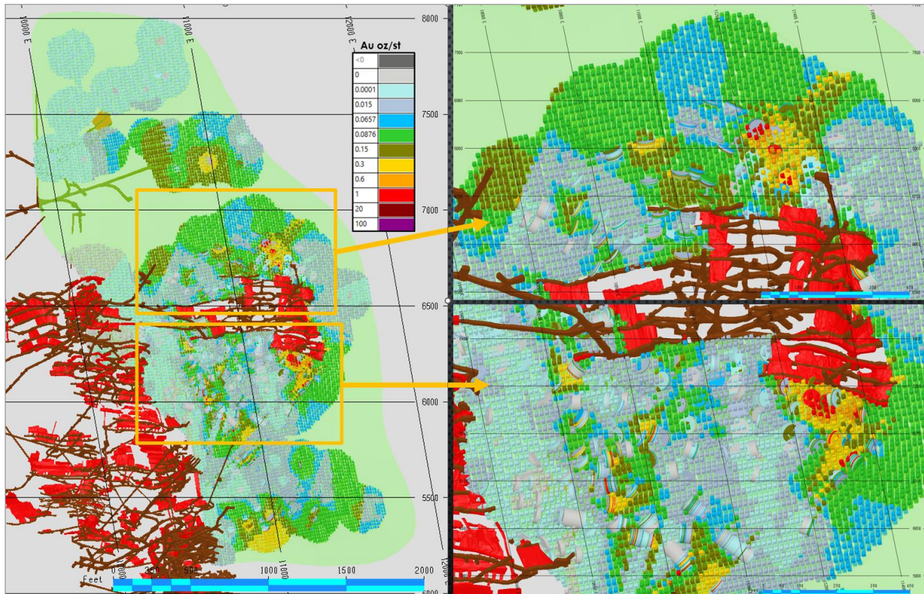
Figure 14.12 Vein 710 vertical longitudinal section (looking north), drillholes, and block model
