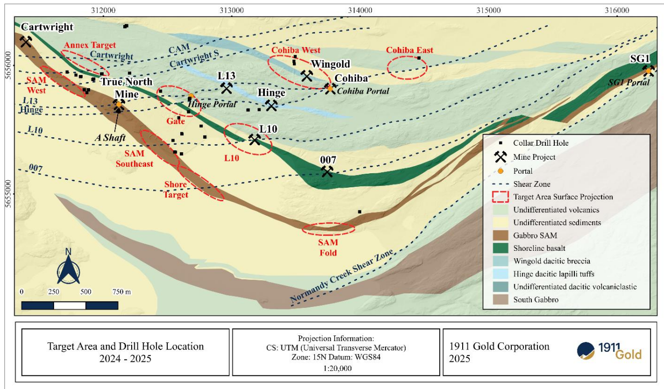
Figure 9.10 True North Mine simplified geology map and drill target areas
