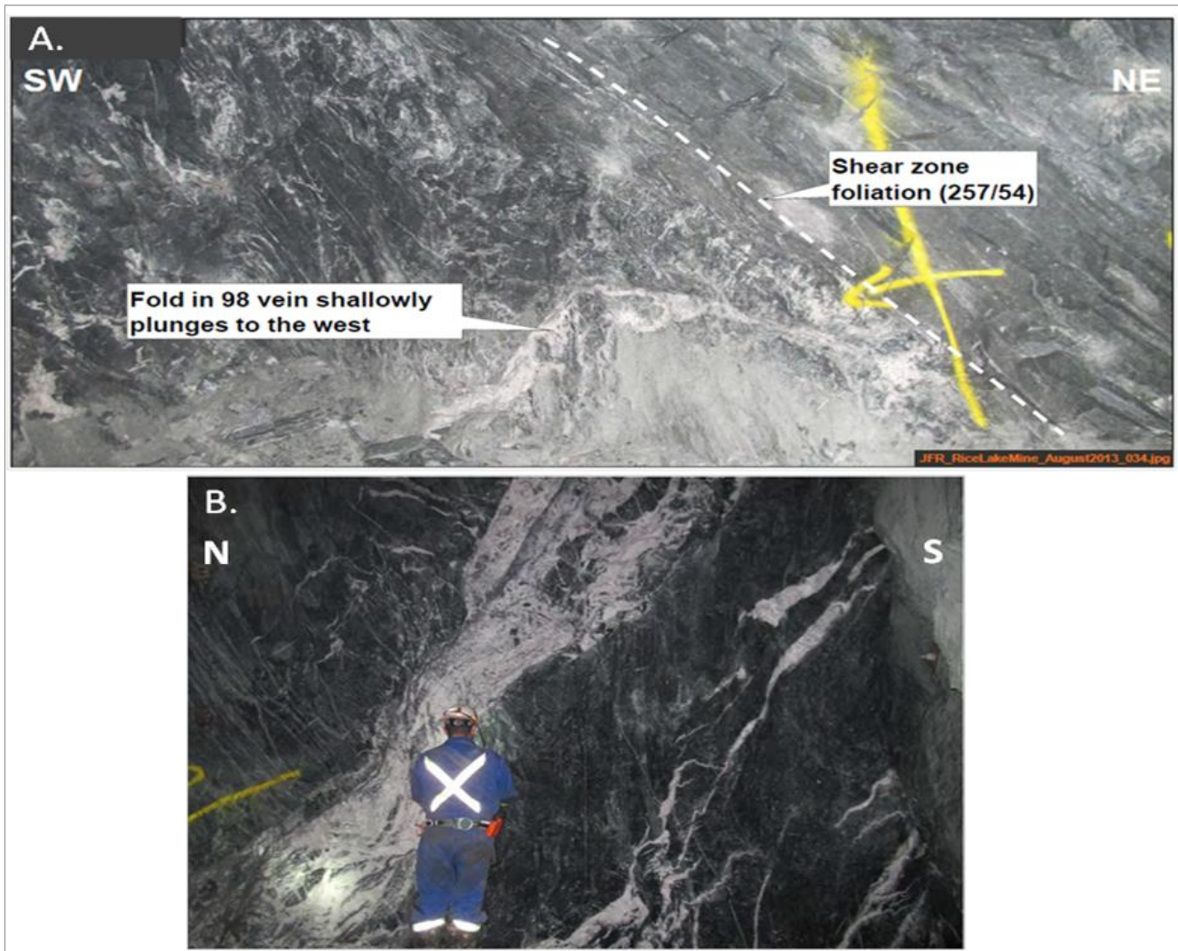
Figure 7.6 Shear zones and quartz veins
