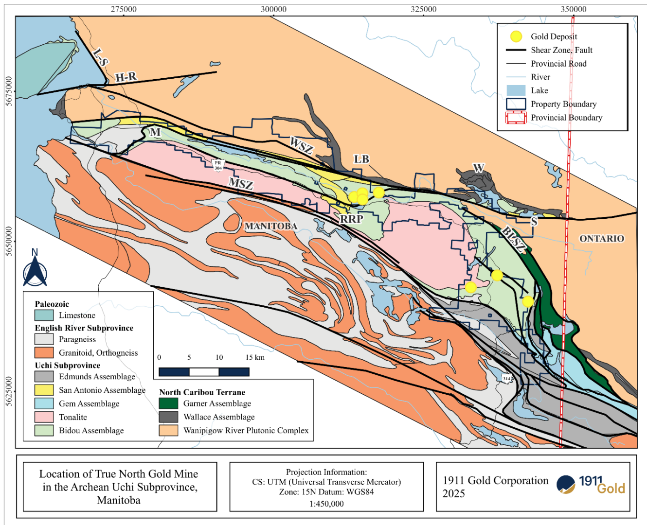
Figure 7.2 Regional geologic map showing the location of True North Gold Project in the Archean Uchi Subprovince, Manitoba
