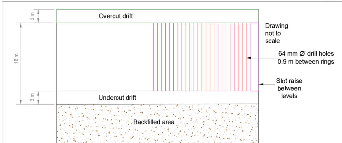
Figure 16.12 Longhole open stope raise and drilling
