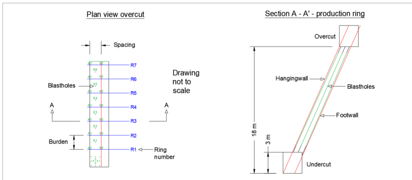
Figure 16.15 Plan view overcut and section A – A' production ring
