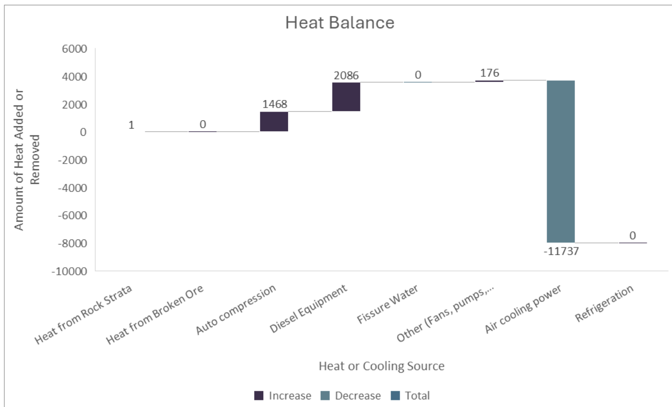
Figure 16.10 Conceptual underground heat load balance
