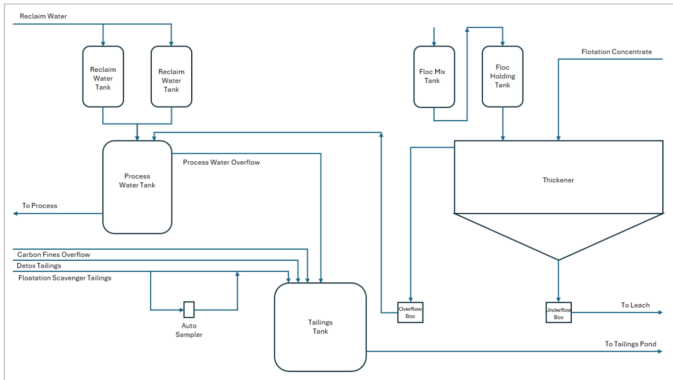
Figure 17.4 1911 Gold processing plant – concentrate thickener circuit
