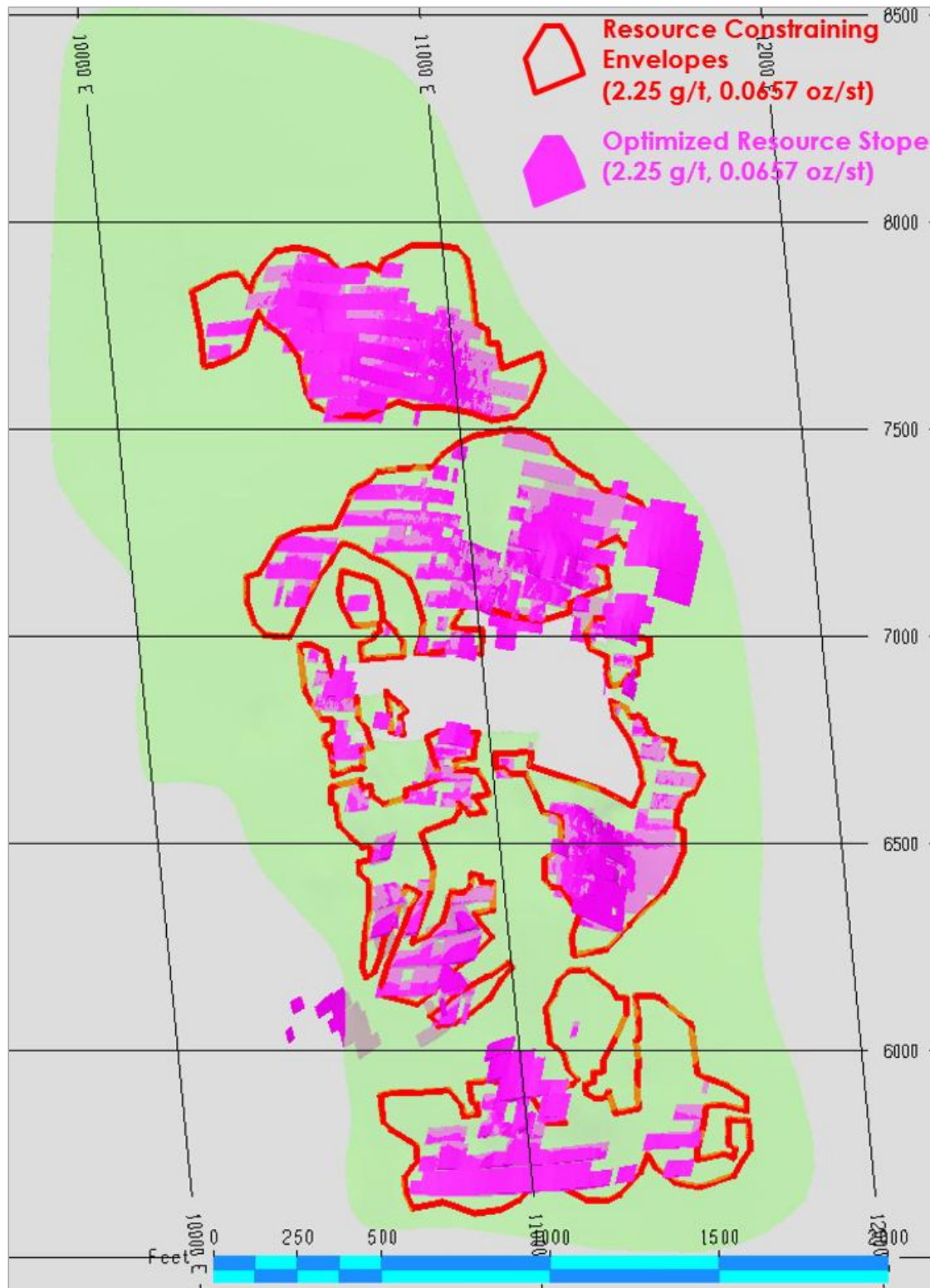
Figure 14.18 Vertical section (looking north), 710-711 Complex Zone, 710 Vein, 0.0657 oz/st Au (2.25 g/t Au) Mineral Resource constraining envelopes (red outline) with overlay of optimized Mineral Resource potential stope shapes (magenta filled outlines)
