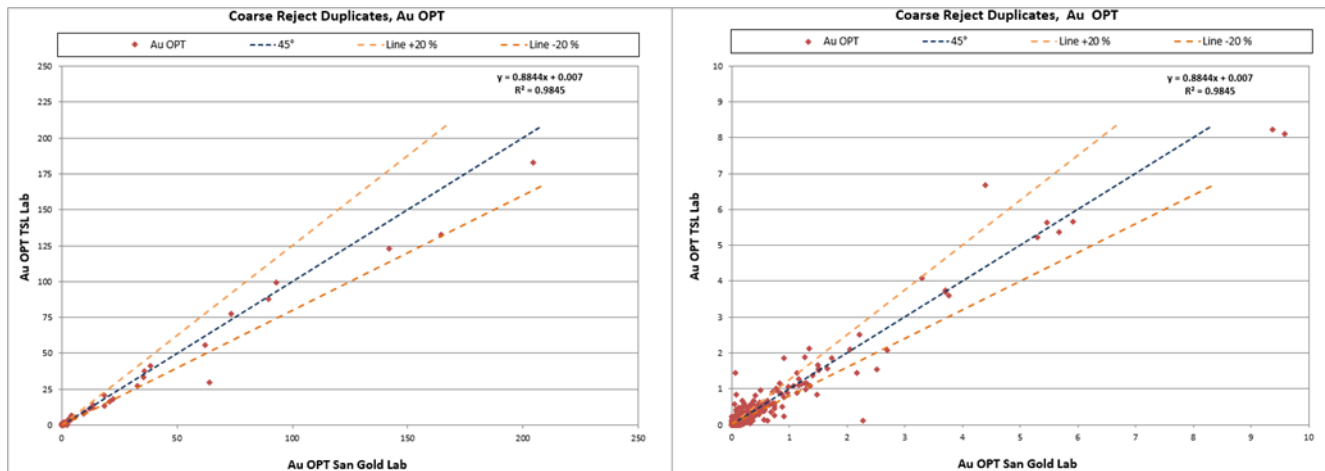
Figure 11.2 Coarse reject duplicates, scatter plot, Au OPT
