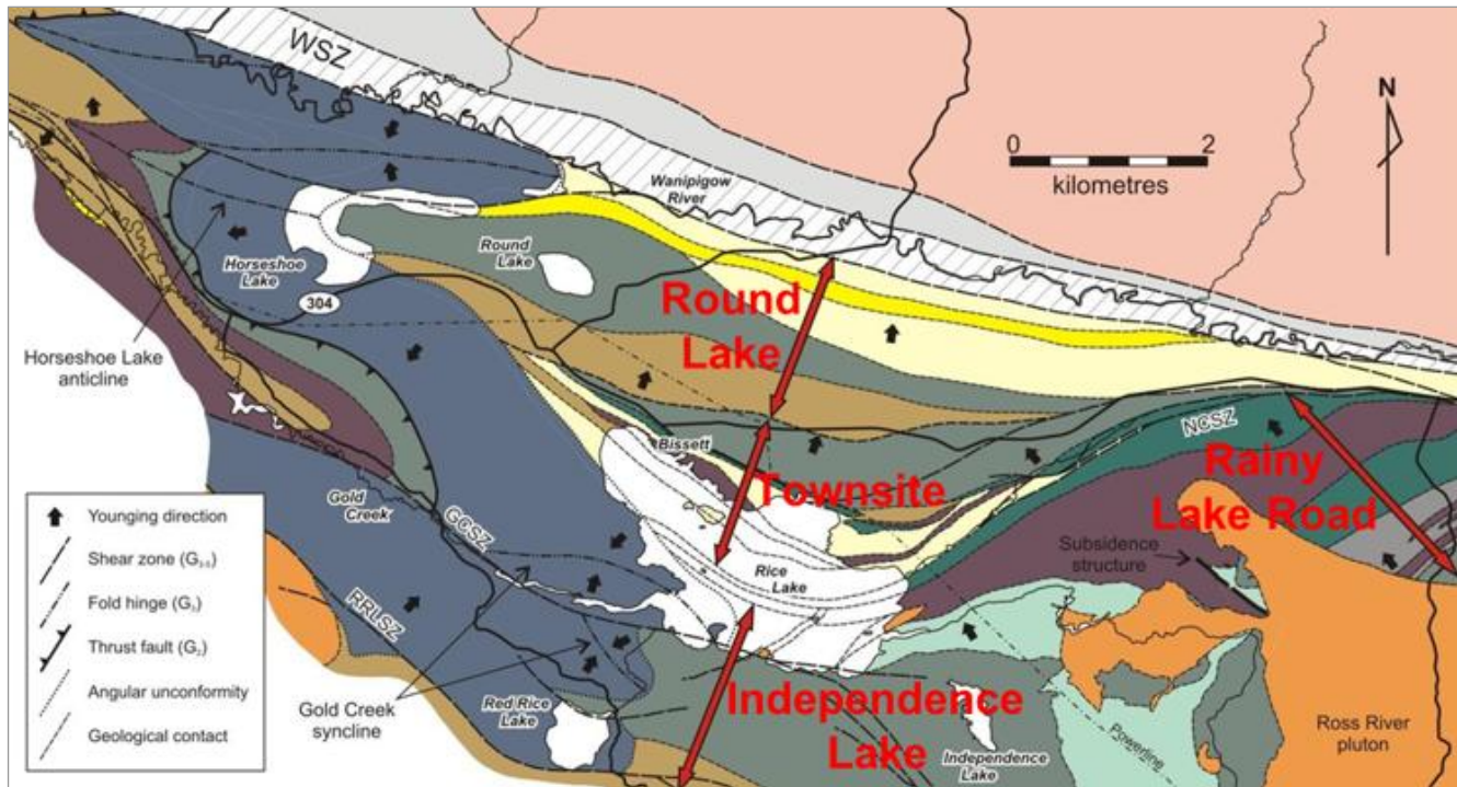
Figure 7.1 Bidou Assemblage – General lithostratigraphic units
