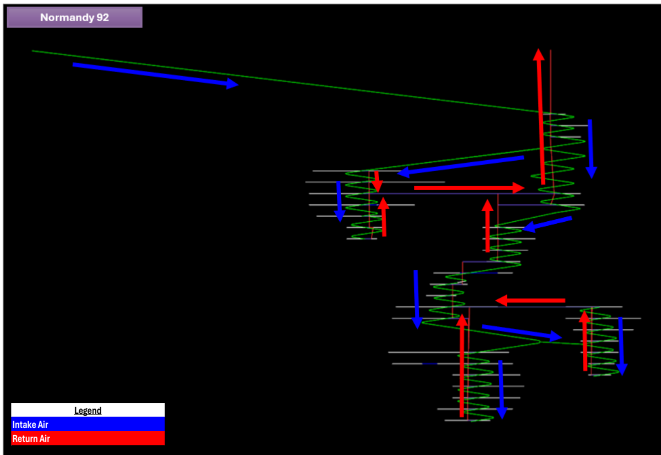
Figure 16.9 Conceptual ventilation flow – Normandy 92 (SG-3) (looking north)
