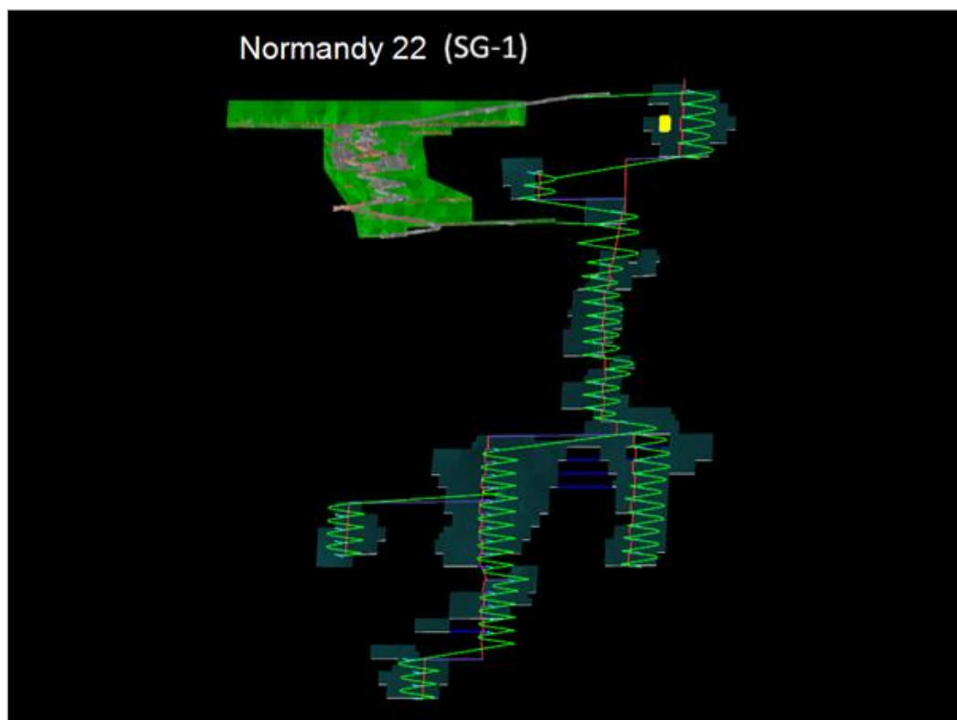
Figure 16.18 Normandy 22 (SG-1) underground mine design (looking north)
