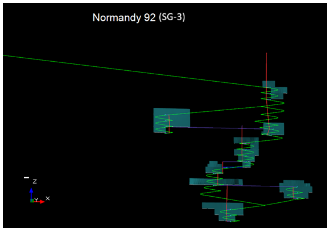
Figure 16.19 Normandy 92 (SG-3) underground mine design (looking north)
