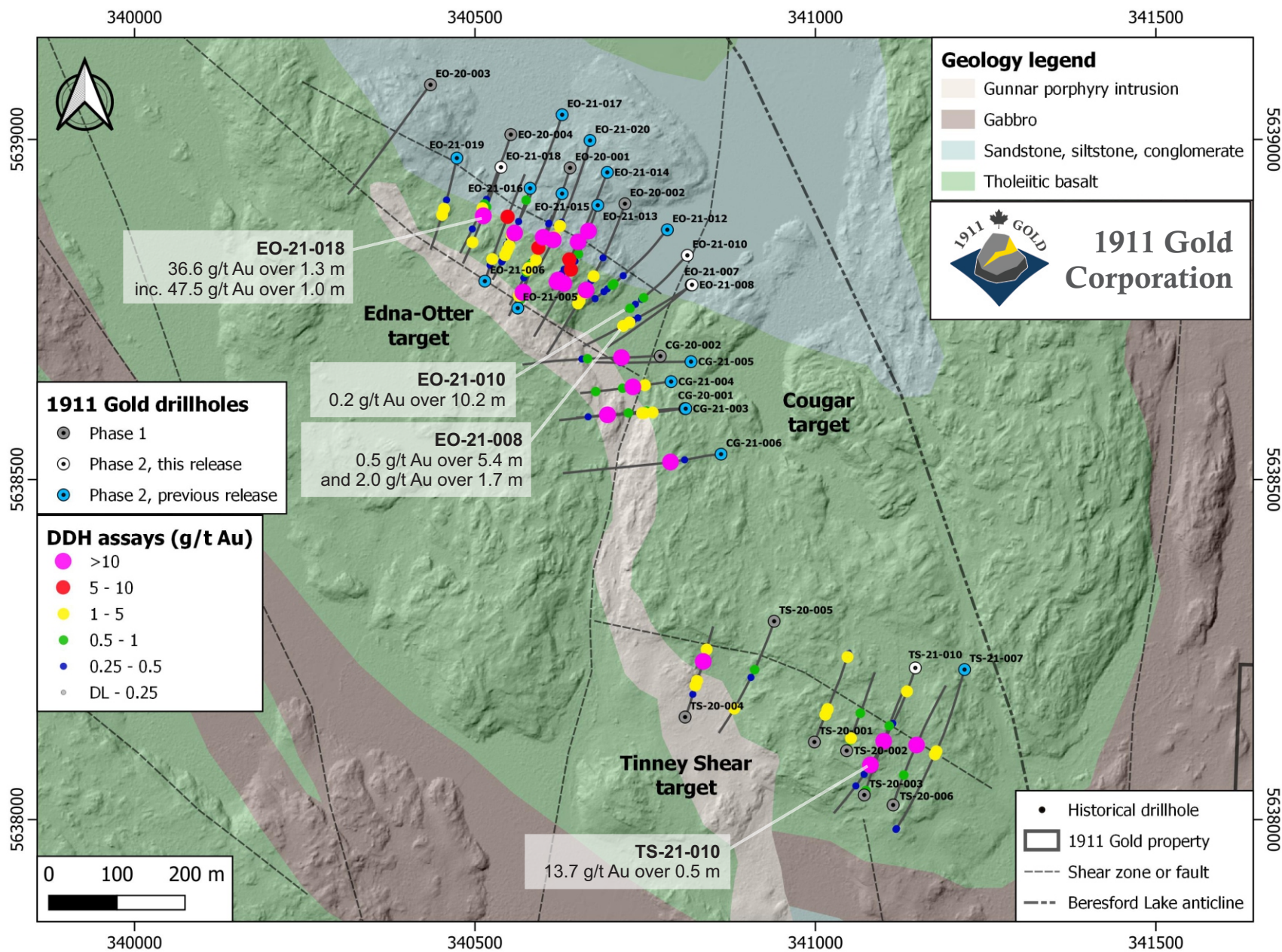
Figure 1: Plan view of Tinney project showing drillhole locations and down-hole assay results; base map is LiDAR bare-earth surface with simplified geology drape.
