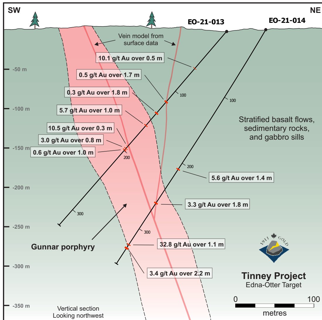
Figure 3: Geological cross section showing drillholes EO-21-013 and EO-21-014, the Gunnar porphyry, vein model from surface data, and new gold intercepts from 2021 drilling.
