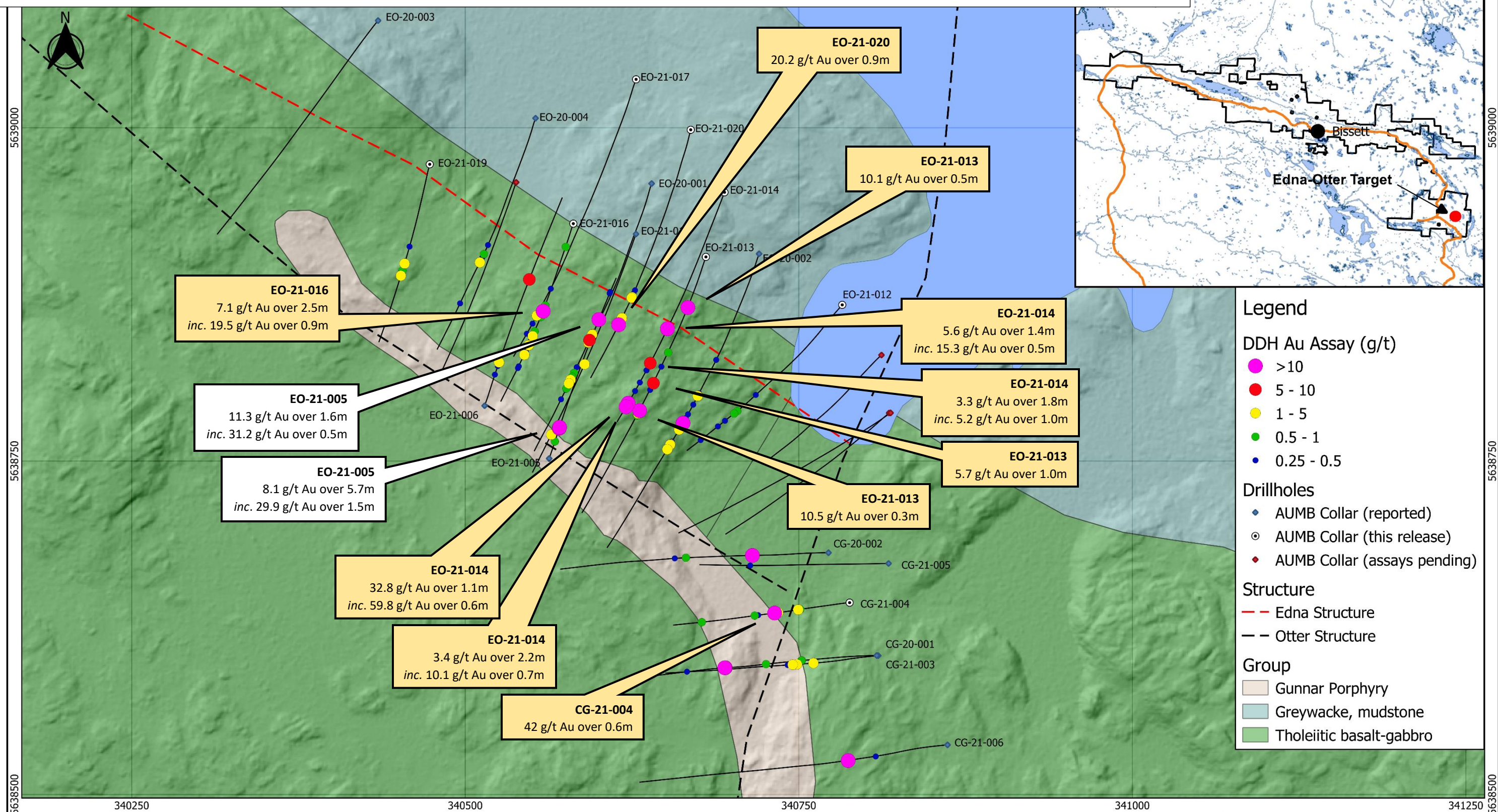
Figure 2: Detailed plan of the northern portion of the Gunnar porphyry showing 2020-2021 drillholes and new drill intercepts reported in this release (yellow call-outs)
