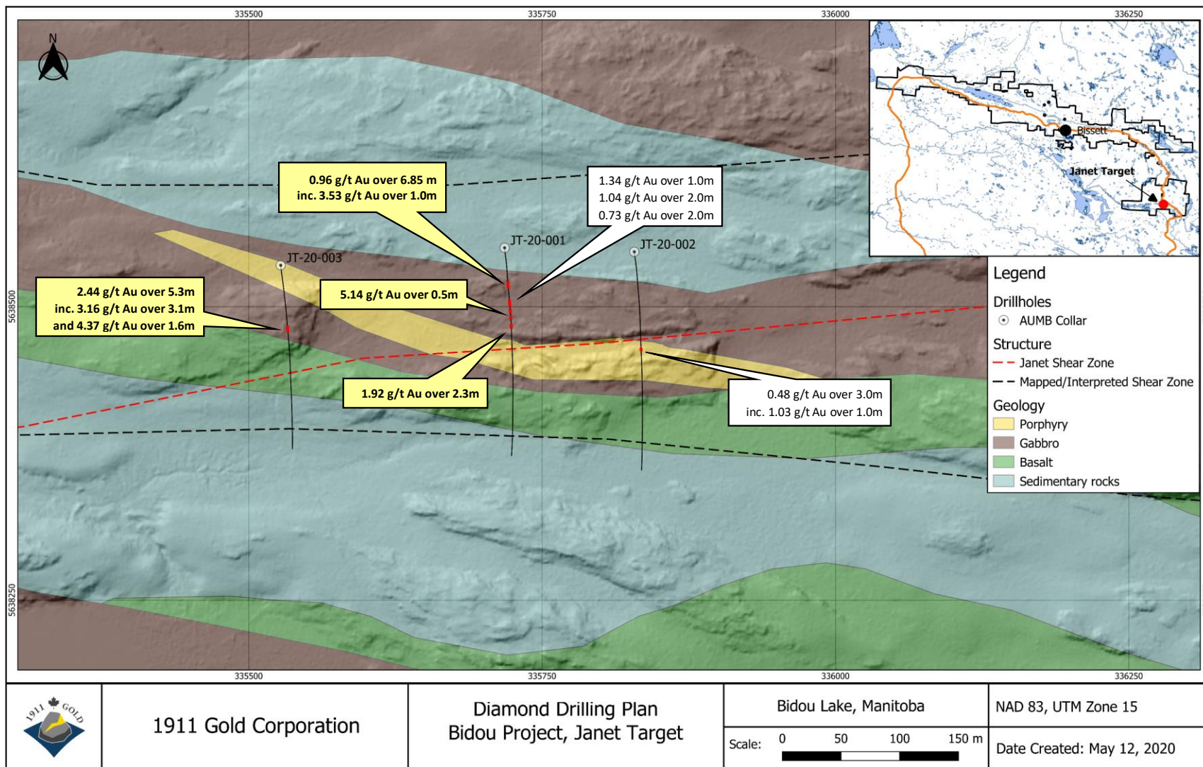
Figure 5: Plan map of the Janet (JT) target, showing drillhole locations and major structures. Map base is a shaded-relief LiDAR DEM with bedrock geology drape. Drillhole intercepts of less than 1 g/t Au over less than 1.0 m are omitted for clarity (refer to Table 1 for complete listing).
