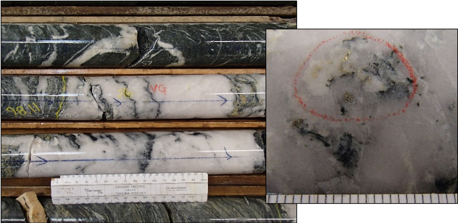
Figure 3: Drillcore photos of laminated shear vein and visible gold from DDH BS-19-001.
