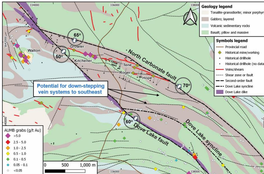
Figure 6: Simplified map of the Central Manitoba mine area showing the general geology and structure, with the historically-defined vein and shear structures, and the locations of previous drillholes.
